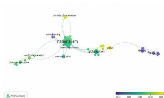
Gambar 4 Overlay Visualization Tren Topik Penelitian
