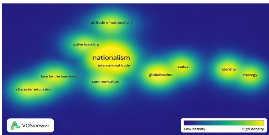
Gambar 5 Density Visualization Tema Penelitian
