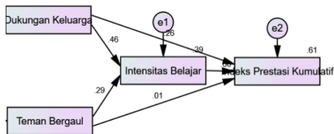
Gambar 1. Path Diagram
