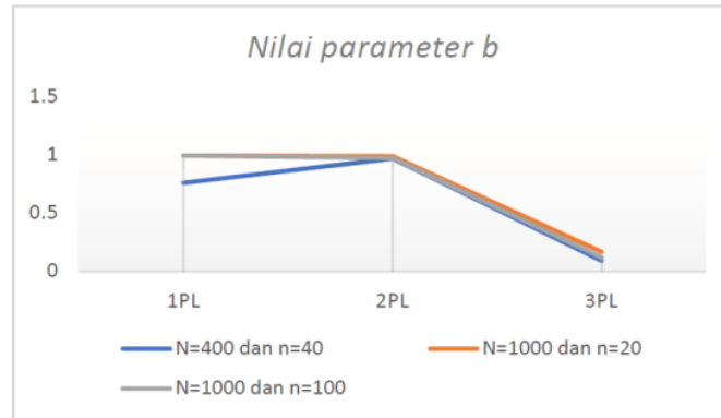
Figure 8 Graph of parameter recapitulation results b
