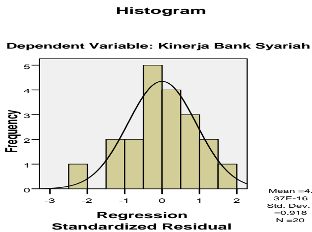
Gambar 4. Histogram (BRIS)
